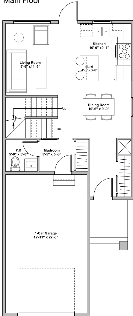
Main Floor
