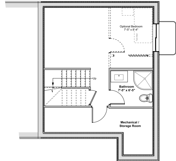
Basement
